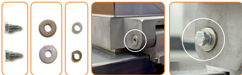
Step 8: Fix the grid frame with the short screws, washers and spring washers on both sides
